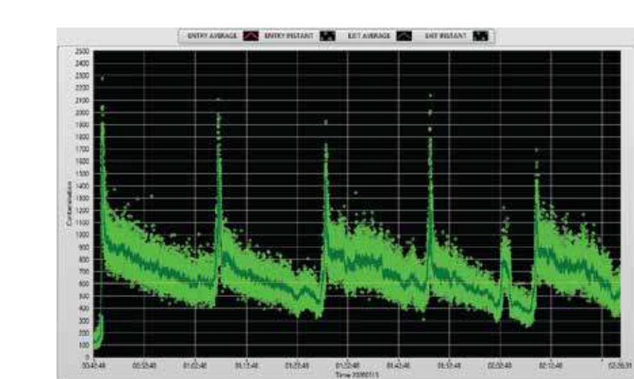
Pollution trend of coils surface showing typical cold mill contamination
