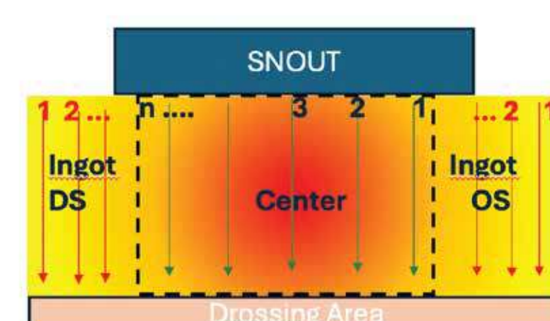
Example of the sequence for racking
