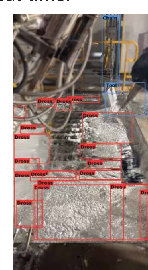
Example of AI image analysis on pot surface accessible by robot
