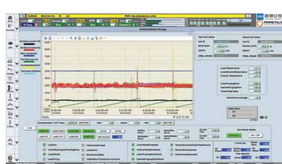
HMI of line PLC - Contamination data & Process parameters in real time
